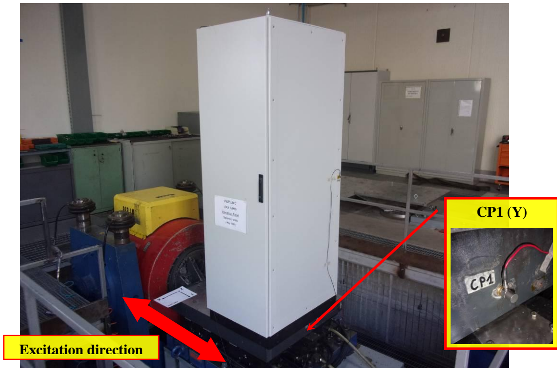
Photo 2: Test configuration for seismic test in Y direction
