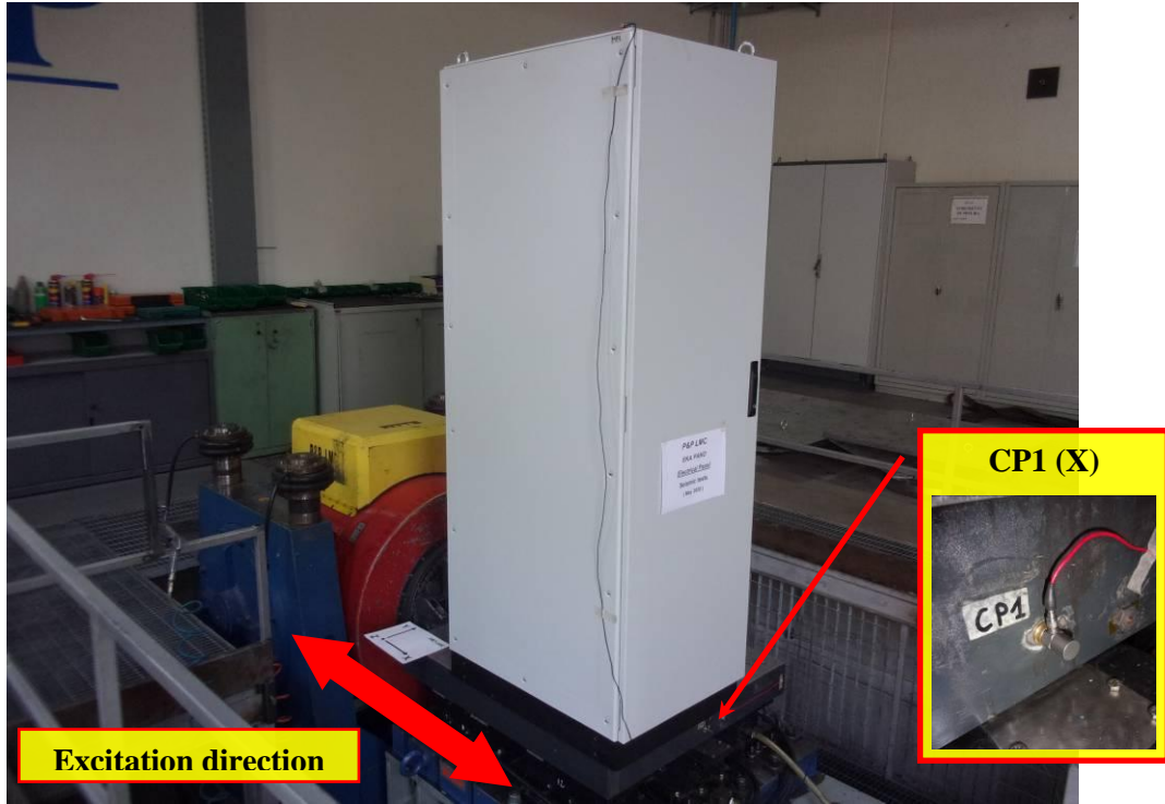
Photo 1: Test configuration for seismic test in X direction
